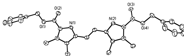
Figure 1. View of the molecular structure of 18 in the crystal. Hydrogen atoms have been omitted for clarity; ellipsoids show 50% occupancy.
